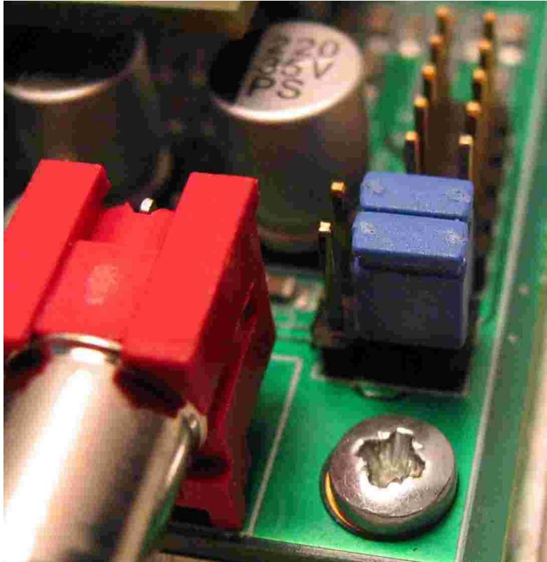
J11 - Jumper position for RCA audio input
