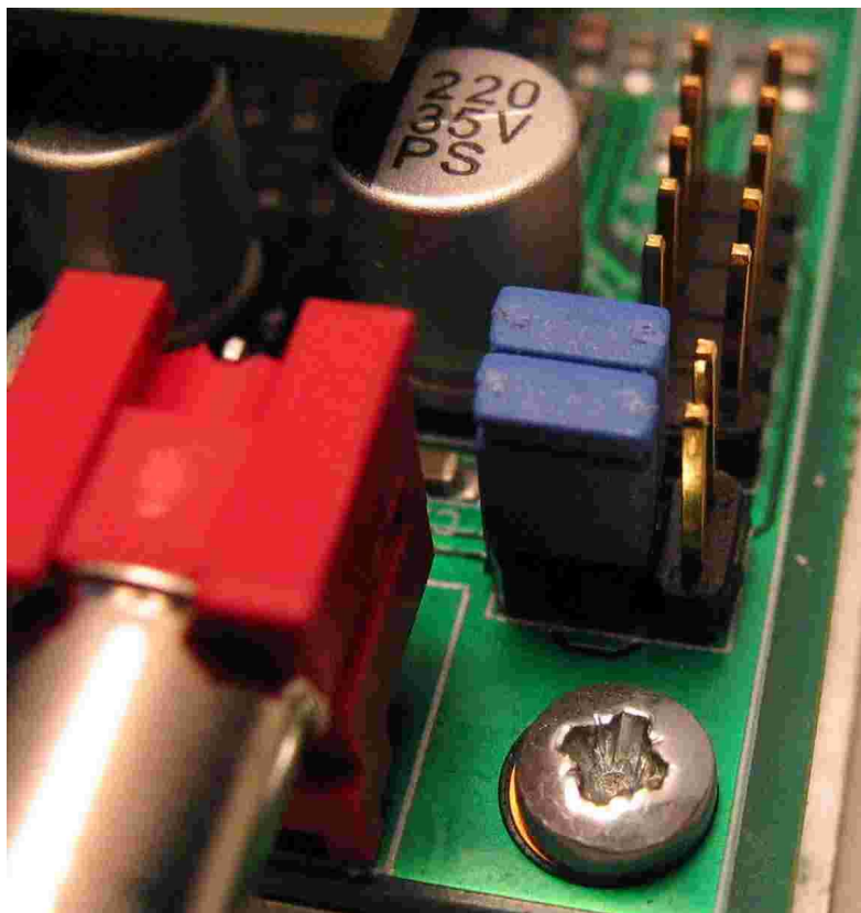
J11 - Jumper position for RCA audio output
